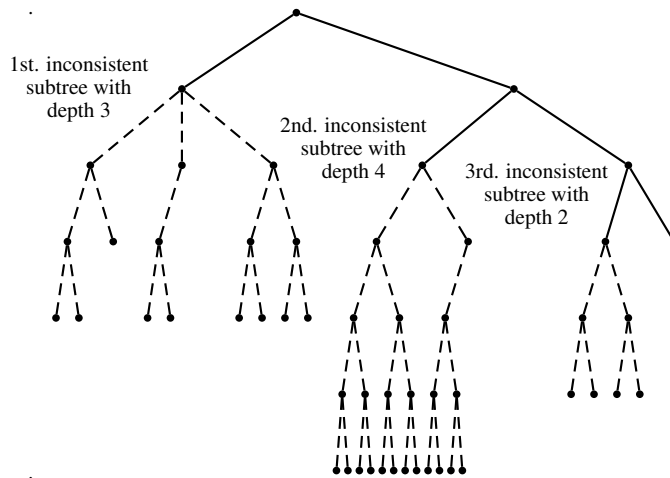
Figure 2. Inconsistent subtrees in backtrack search.
