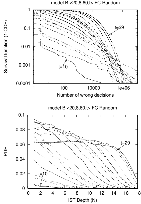
Figure 6. The progression from heavy-tailed regime to non-heavy-tailed regime for FC Random algorithm on instances of model B \langle 20, 8, 60, t \rangle . (The value of t increases by 1 between curves.)
