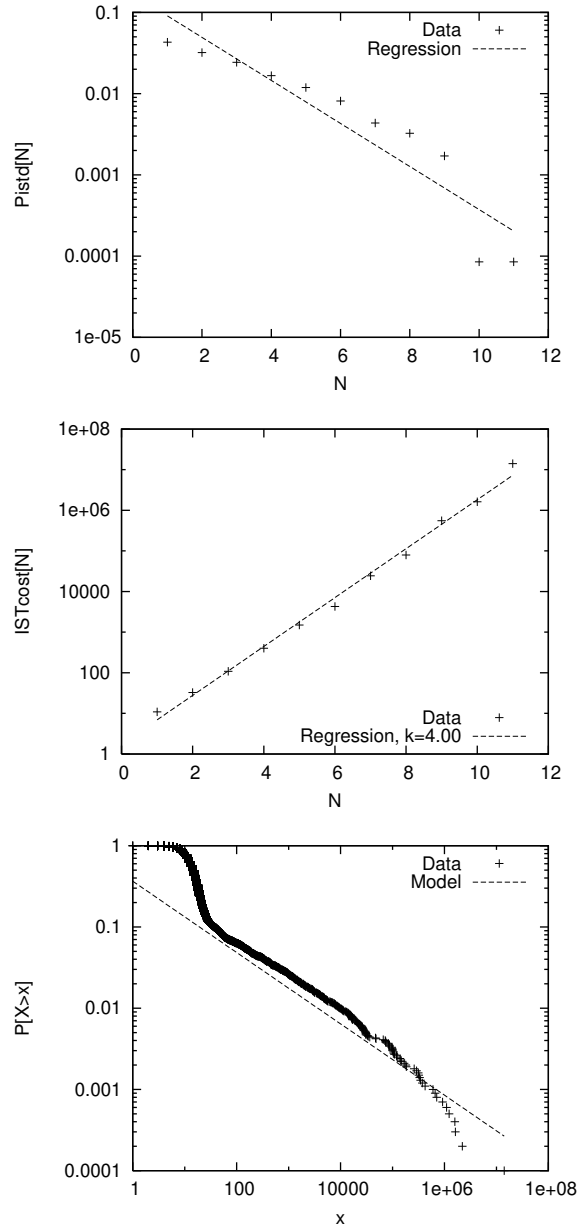
Figure 11. Regressions for the estimation of B1=0.167 , B2=0.610 (top plot; quality of fit R^2 = 0.86 ), and k = 4.00 (middle plot; R^2 = 0.99 ) and comparison of lower bound based on the theoretical model with empirical data (bottom plot). We have \alpha = B_2/\ln(k) = 0.439 from our model; \alpha = 0.443 directly from runtime data. Model E(17, 8, 0.07) , using BT-random .
