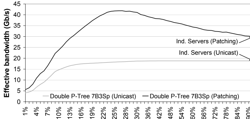
Fig. 3. Double P-Tree Effective Bandwidth & Proxy Storage Capacity
