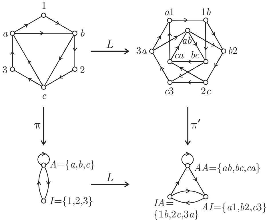
Figure 3: The line and quotient digraph operations commute.
