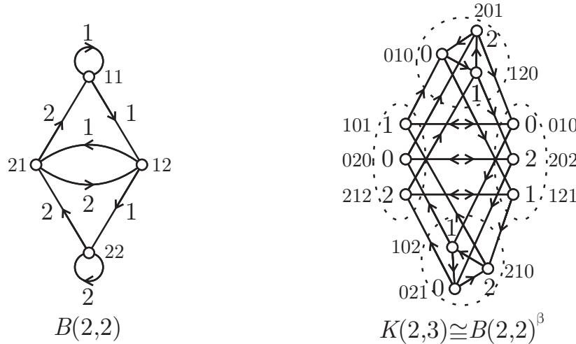
Figure 2: K(2,3) as a lifted digraph of the base digraph B(2,2) .
