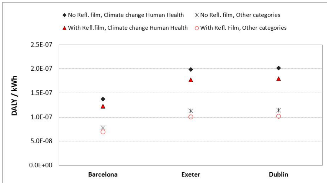
Figure 2. ReCiPe endpoint/with characterization: a) The contribution of each component 3 to the total impact of material manufacturing (43 modules; configuration with reflective film) according to climate change/human health, ozone depletion, human toxicity, photochemical oxidant formation, particulate matter formation and ionising radiation (DALY); b) DALY per kWh of produced electricity for Barcelona, Exeter and Dublin, configurations with/without reflective film, 25-years lifespan, studied categories: i) climate change/human health and ii) other categories (ozone depletion, human toxicity, photochemical oxidant formation, particulate matter formation and ionising radiation) (Source: [35]).
