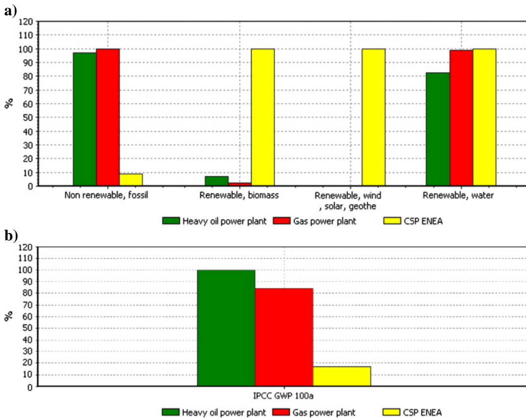
Figure 4. Results from the study of Piemonte et al. [62]. LCA comparisons (heavy-oil power plant, gas power plant vs. CSP ENEA) based on: a) CED and b) GWP 100a (IPCC) (Source: [62]).
