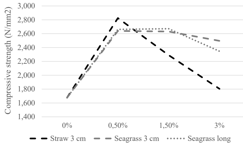
Figure 1. Compressive strength of the adobe bricks according to the fibre length (3 cm straw/seagrass, long seagrass) and fibre content (0, 0.5, 1.5, and 3%).
