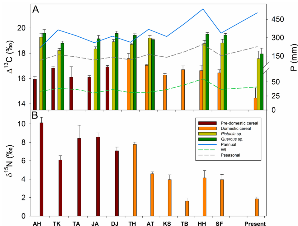
Figure 2. \Delta^{13}\text{C} and \delta^{15}\text{N} of archaeobotanical samples recovered at each site
