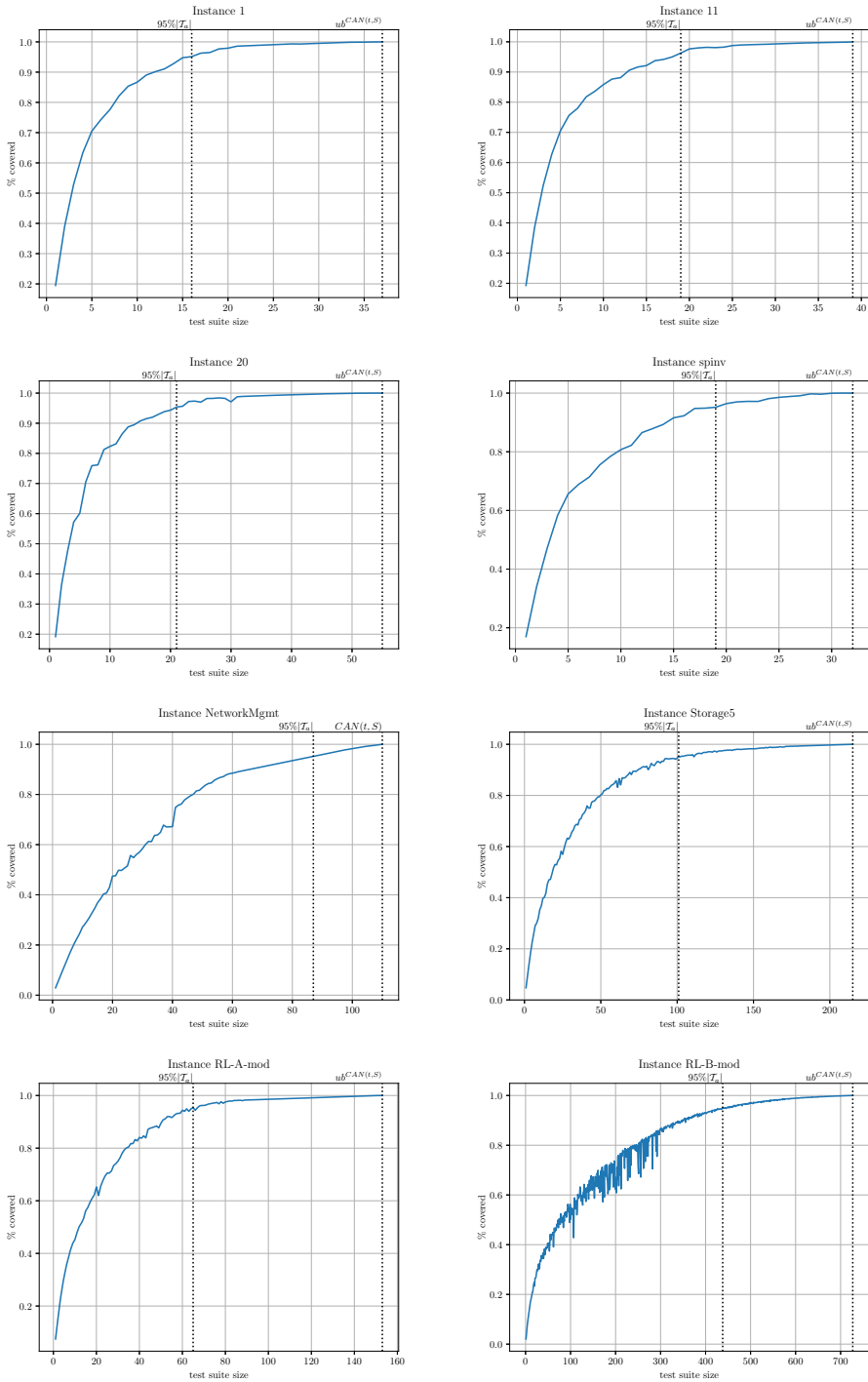
Fig. 1 Number of tests required to reach a certain coverage percentage for the ti-open-wbo-inc approach
