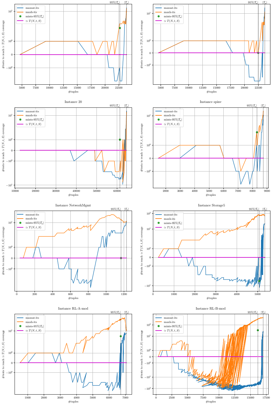
Fig. 2 Comparison of the required number of tests for different methods with regards to the number of test used by \cong T(N, t, S) (as base) to cover each number of tuples
