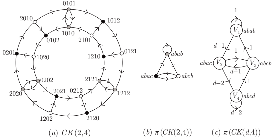
Figure 1: The cyclic Kautz digraph CK(2,4) , its quotient \pi(CK(2,4)) , and the quotient digraph of CK(d,4) .
