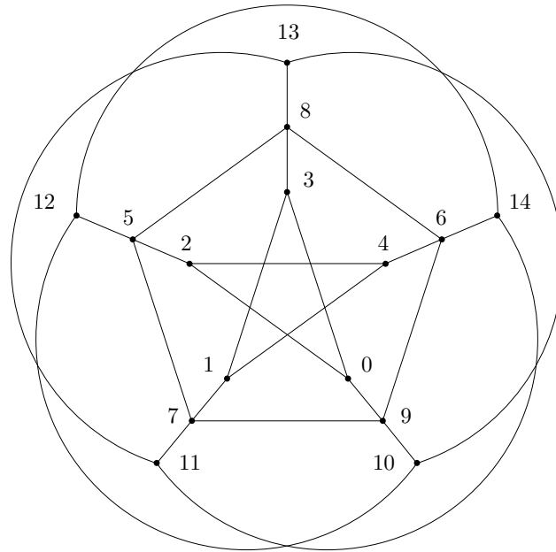
Figure 2: The graph P_3 .
