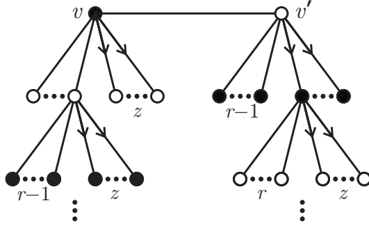
Figure 1: A Moore (r, z) -regular mixed graph hung from an edge.
